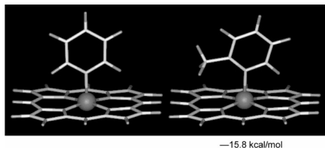
Figure 3. Computation of coordination energy between pyridine and 2-methylpyridine to heme.
